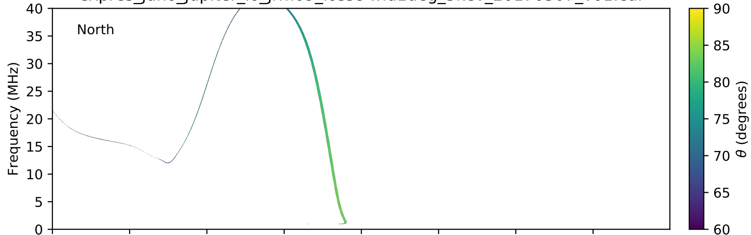
expres_juno_jupiter_io_jrm09_lossc-wid1deg_3kev_20170307_v01.cdf
