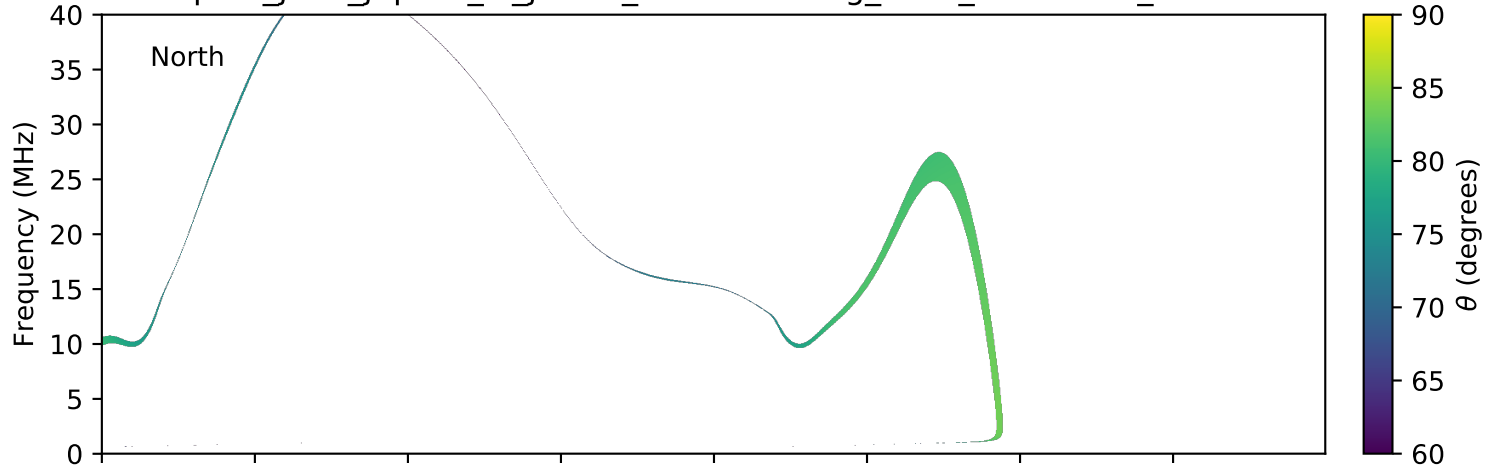
expres_juno_jupiter_io_jrm09_lossc-wid1deg_3kev_20170305_v01.cdf
