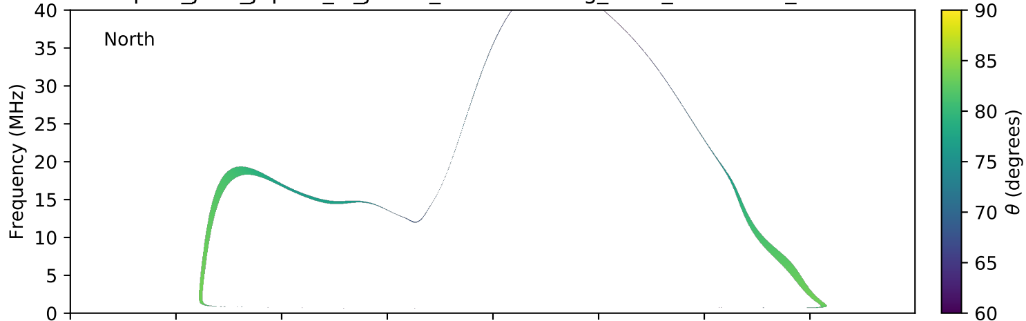
expres_juno_jupiter_io_jrm09_lossc-wid1deg_3kev_20170303_v01.cdf
