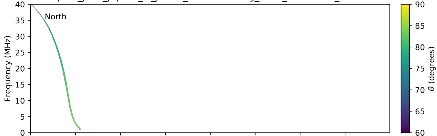
expres_juno_jupiter_io_jrm09_lossc-wid1deg_3kev_20170302_v01.cdf
