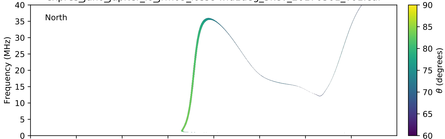
expres_juno_jupiter_io_jrm09_lossc-wid1deg_3kev_20170301_v01.cdf
