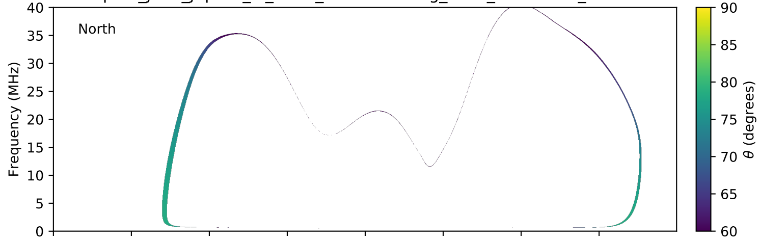
expres_juno_jupiter_io_isaac_lossc-wid1deg_9kev_20170326_v01.cdf
