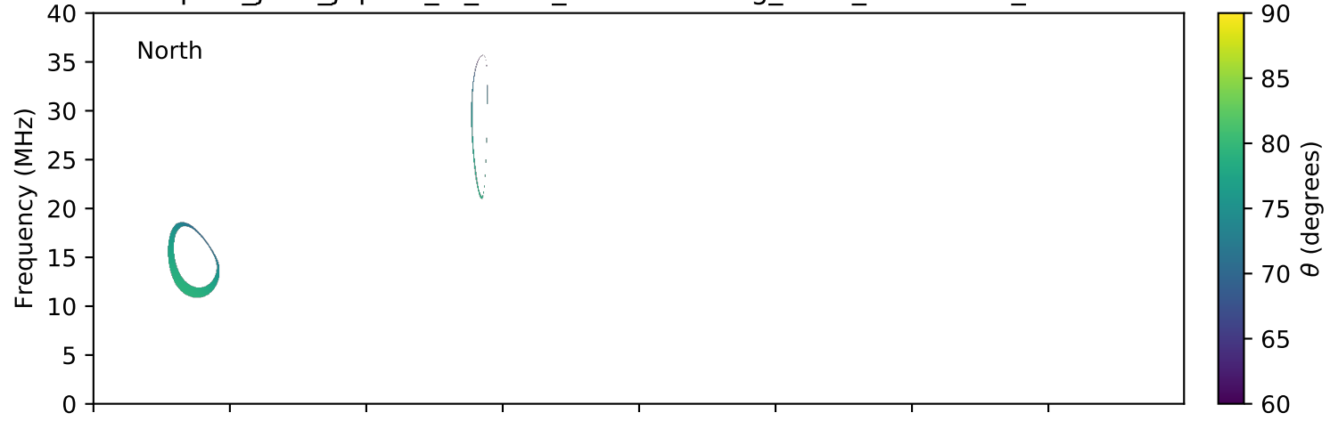
expres_juno_jupiter_io_isaac_lossc-wid1deg_5kev_20170327_v01.cdf
