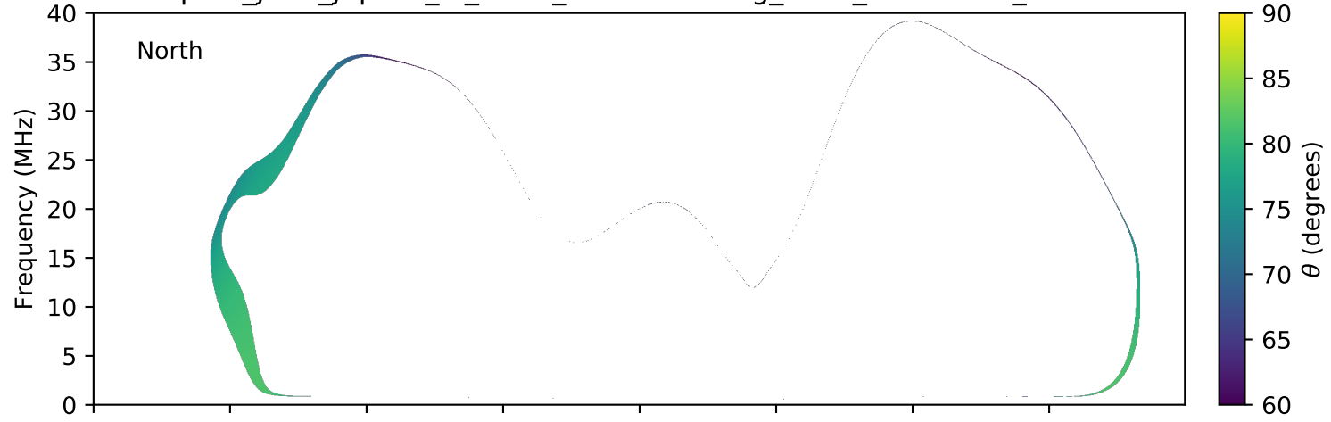
expres_juno_jupiter_io_isaac_lossc-wid1deg_5kev_20170326_v01.cdf
