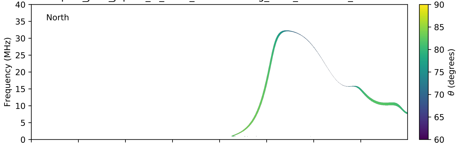
expres_juno_jupiter_io_isaac_lossc-wid1deg_3kev_20170331_v01.cdf
