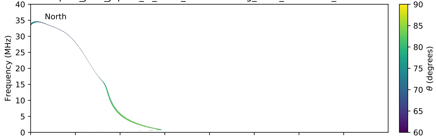
expres_juno_jupiter_io_isaac_lossc-wid1deg_3kev_20170330_v01.cdf
