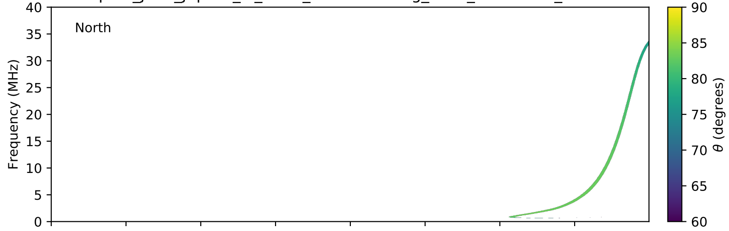
expres_juno_jupiter_io_isaac_lossc-wid1deg_3kev_20170329_v01.cdf
