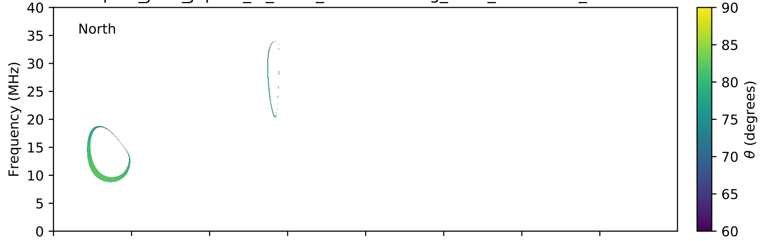
expres_juno_jupiter_io_isaac_lossc-wid1deg_3kev_20170327_v01.cdf
