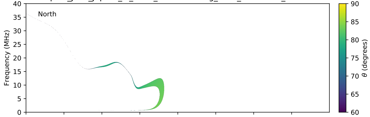
expres_juno_jupiter_io_isaac_lossc-wid1deg_3kev_20170323_v01.cdf
