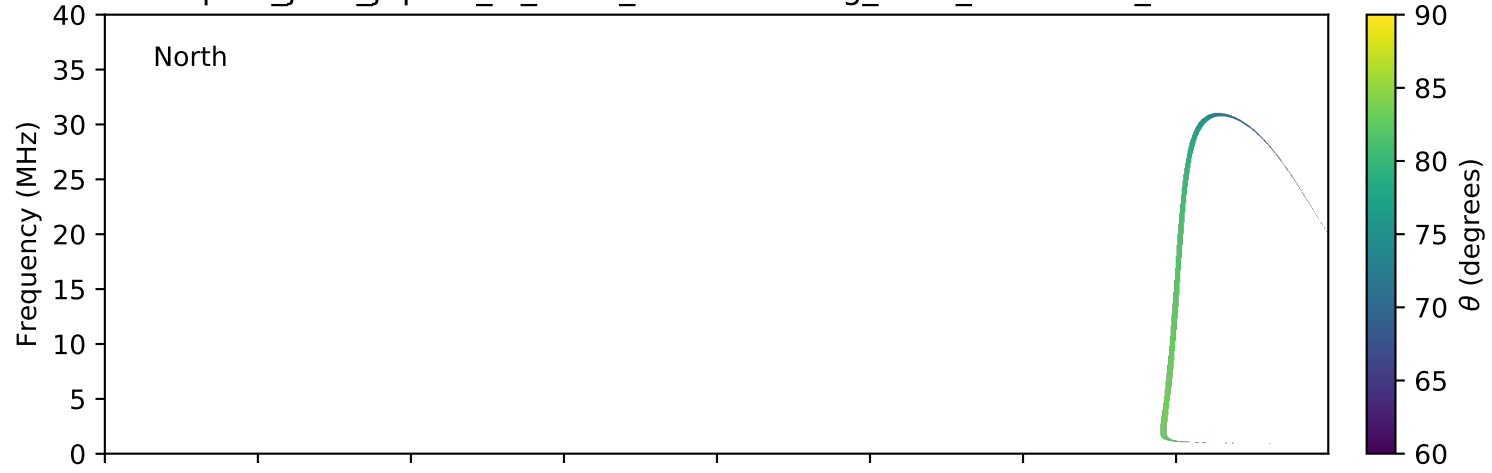
expres_juno_jupiter_io_isaac_lossc-wid1deg_3kev_20170320_v01.cdf
