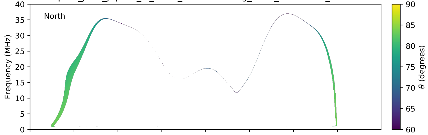
expres_juno_jupiter_io_isaac_lossc-wid1deg_3kev_20170319_v01.cdf
