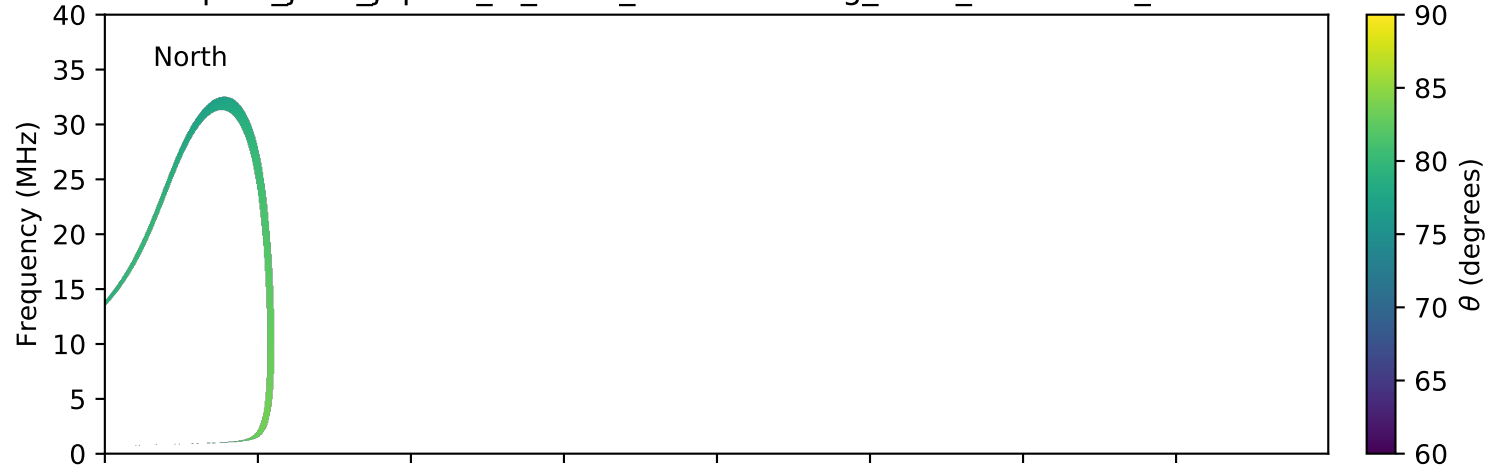
expres_juno_jupiter_io_isaac_lossc-wid1deg_3kev_20170318_v01.cdf
