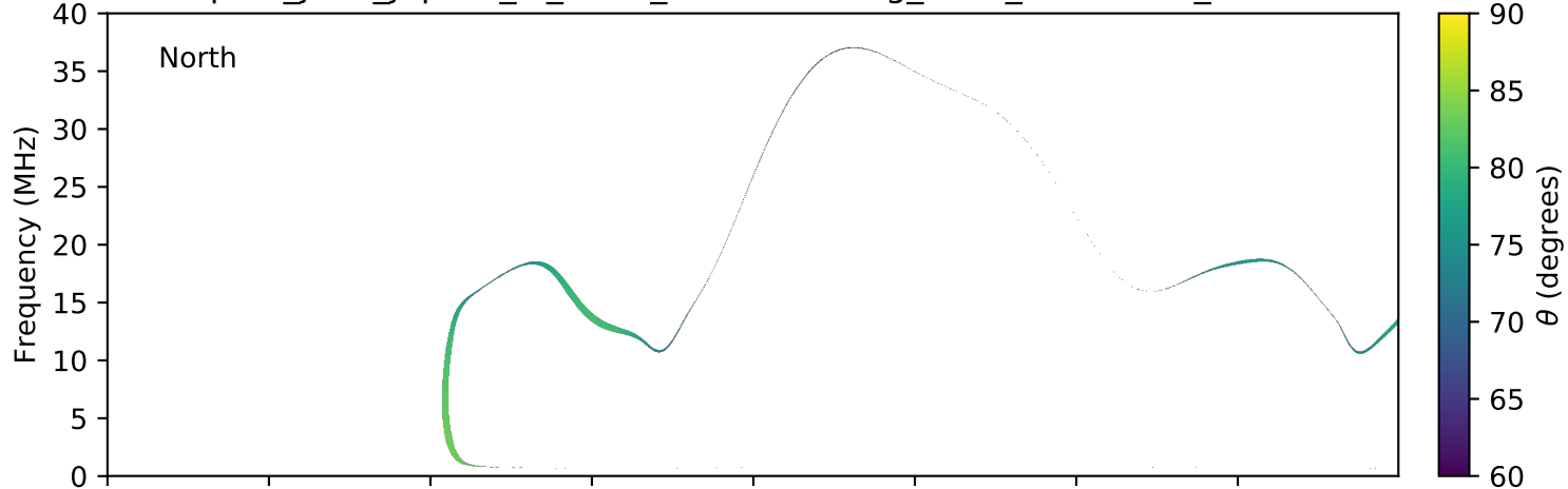
expres_juno_jupiter_io_isaac_lossc-wid1deg_3kev_20170317_v01.cdf
