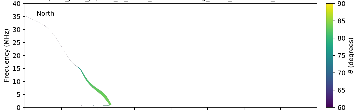
expres_juno_jupiter_io_isaac_lossc-wid1deg_3kev_20170316_v01.cdf
