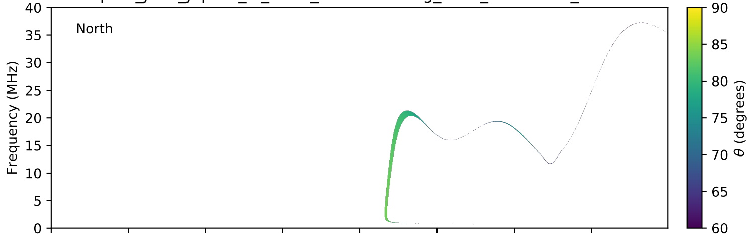
expres_juno_jupiter_io_isaac_lossc-wid1deg_3kev_20170315_v01.cdf
