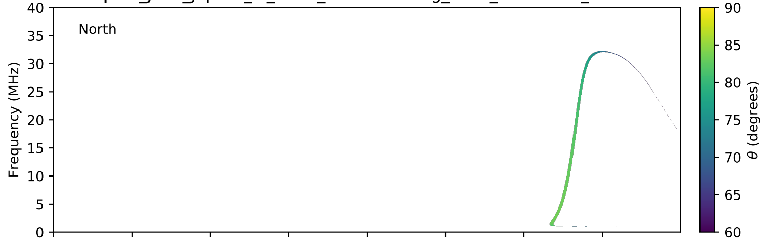
expres_juno_jupiter_io_isaac_lossc-wid1deg_3kev_20170313_v01.cdf
