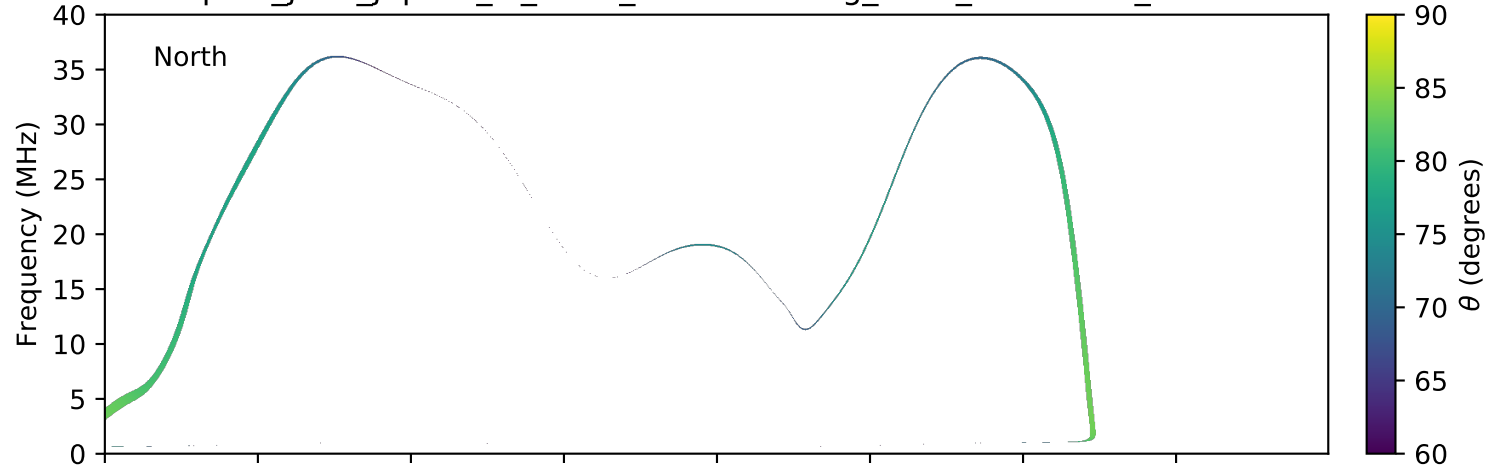
expres_juno_jupiter_io_isaac_lossc-wid1deg_3kev_20170312_v01.cdf
