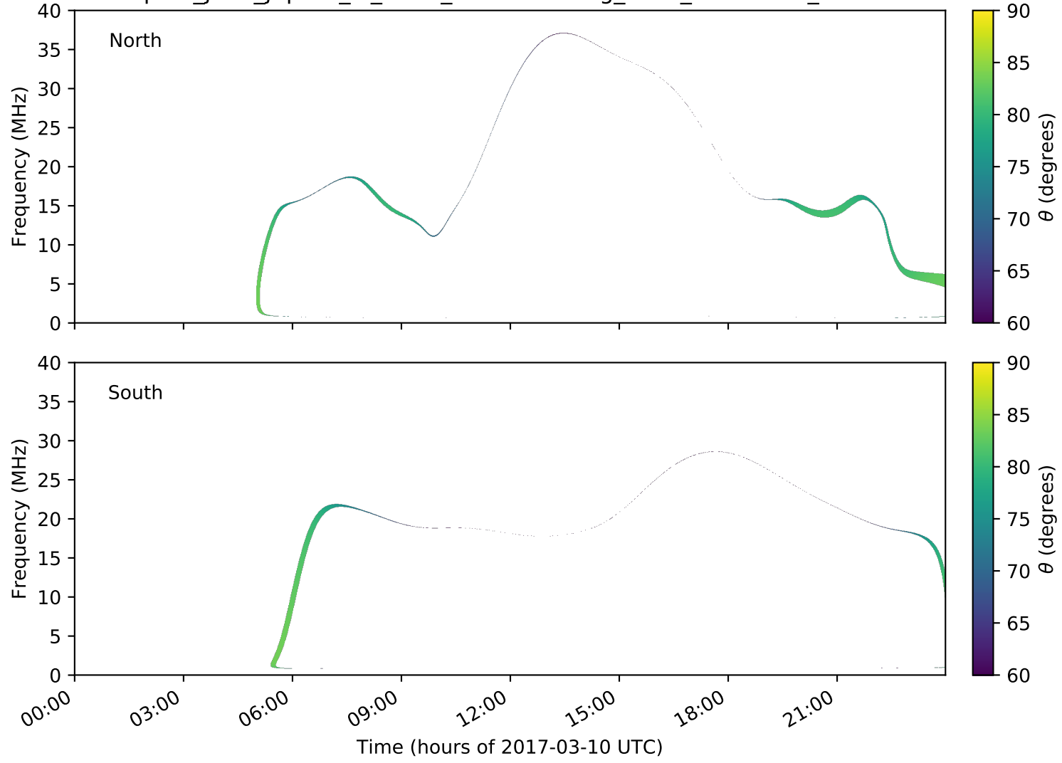
expres_juno_jupiter_io_isaac_lossc-wid1deg_3kev_20170310_v01.cdf
