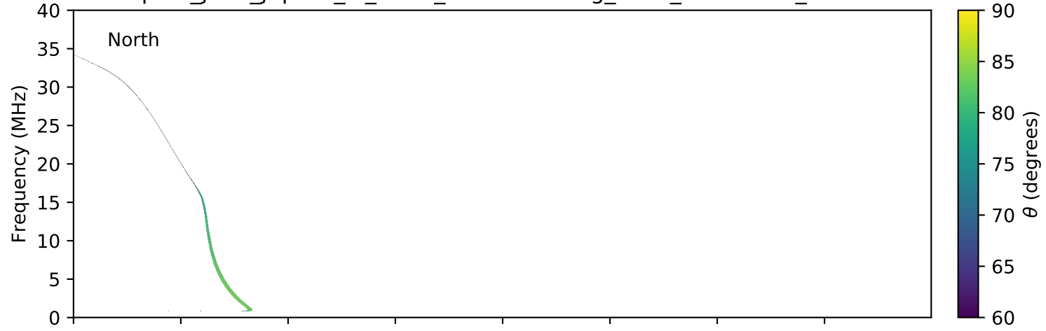
expres_juno_jupiter_io_isaac_lossc-wid1deg_3kev_20170309_v01.cdf
