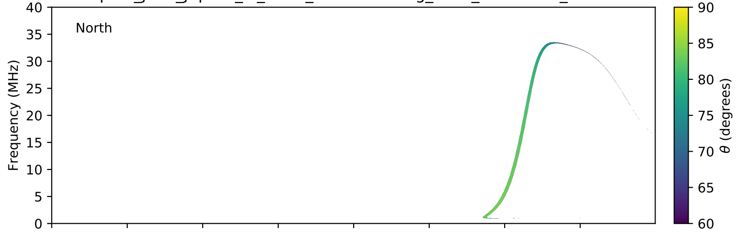
expres_juno_jupiter_io_isaac_lossc-wid1deg_3kev_20170306_v01.cdf
