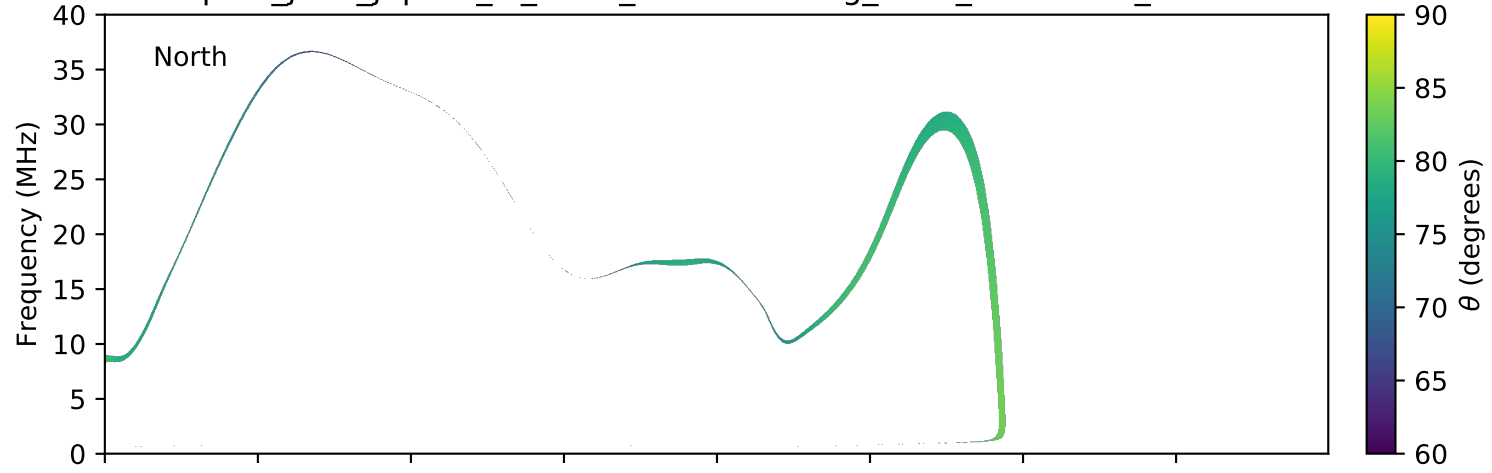
expres_juno_jupiter_io_isaac_lossc-wid1deg_3kev_20170305_v01.cdf
