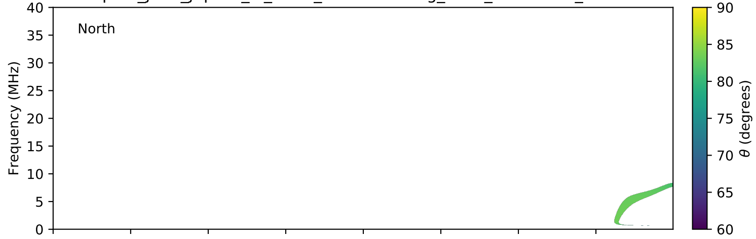
expres_juno_jupiter_io_isaac_lossc-wid1deg_3kev_20170304_v01.cdf
