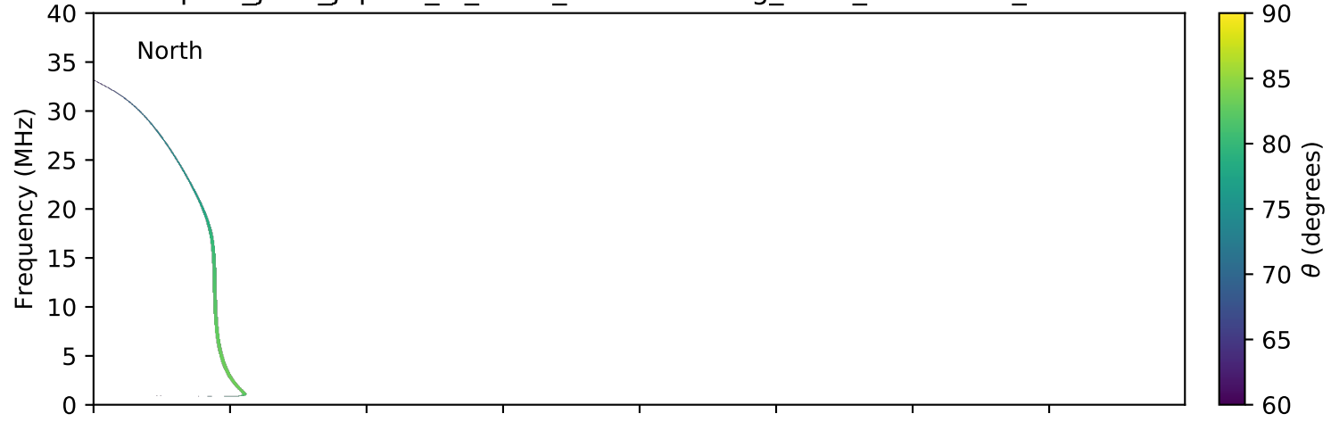
expres_juno_jupiter_io_isaac_lossc-wid1deg_3kev_20170302_v01.cdf
