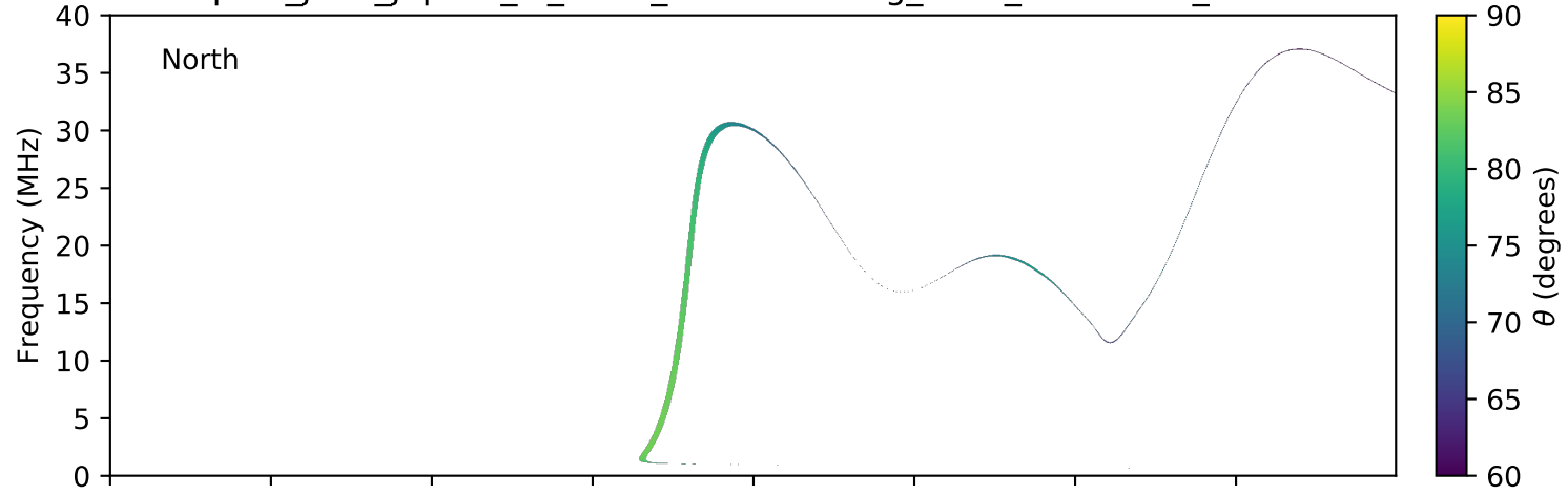
expres_juno_jupiter_io_isaac_lossc-wid1deg_3kev_20170301_v01.cdf
