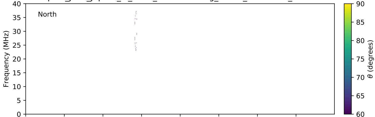
expres_juno_jupiter_io_isaac_lossc-wid1deg_14kev_20170327_v01.cdf
