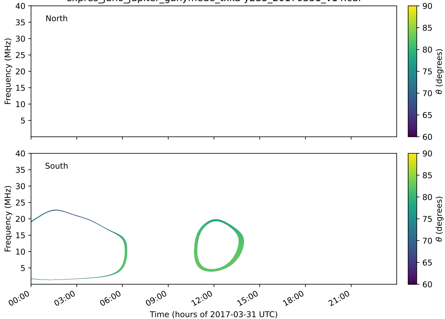
expres_juno_jupiter_ganymede_txka-y235_20170331_v14.cdf
