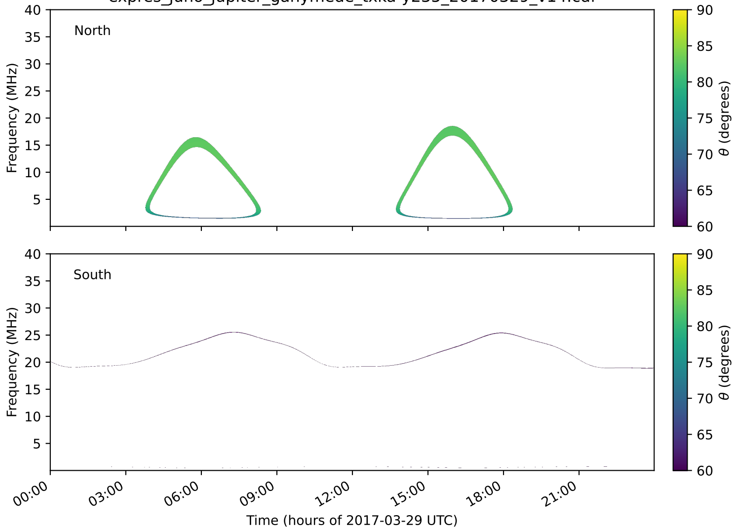
expres_juno_jupiter_ganymede_txka-y235_20170329_v14.cdf
