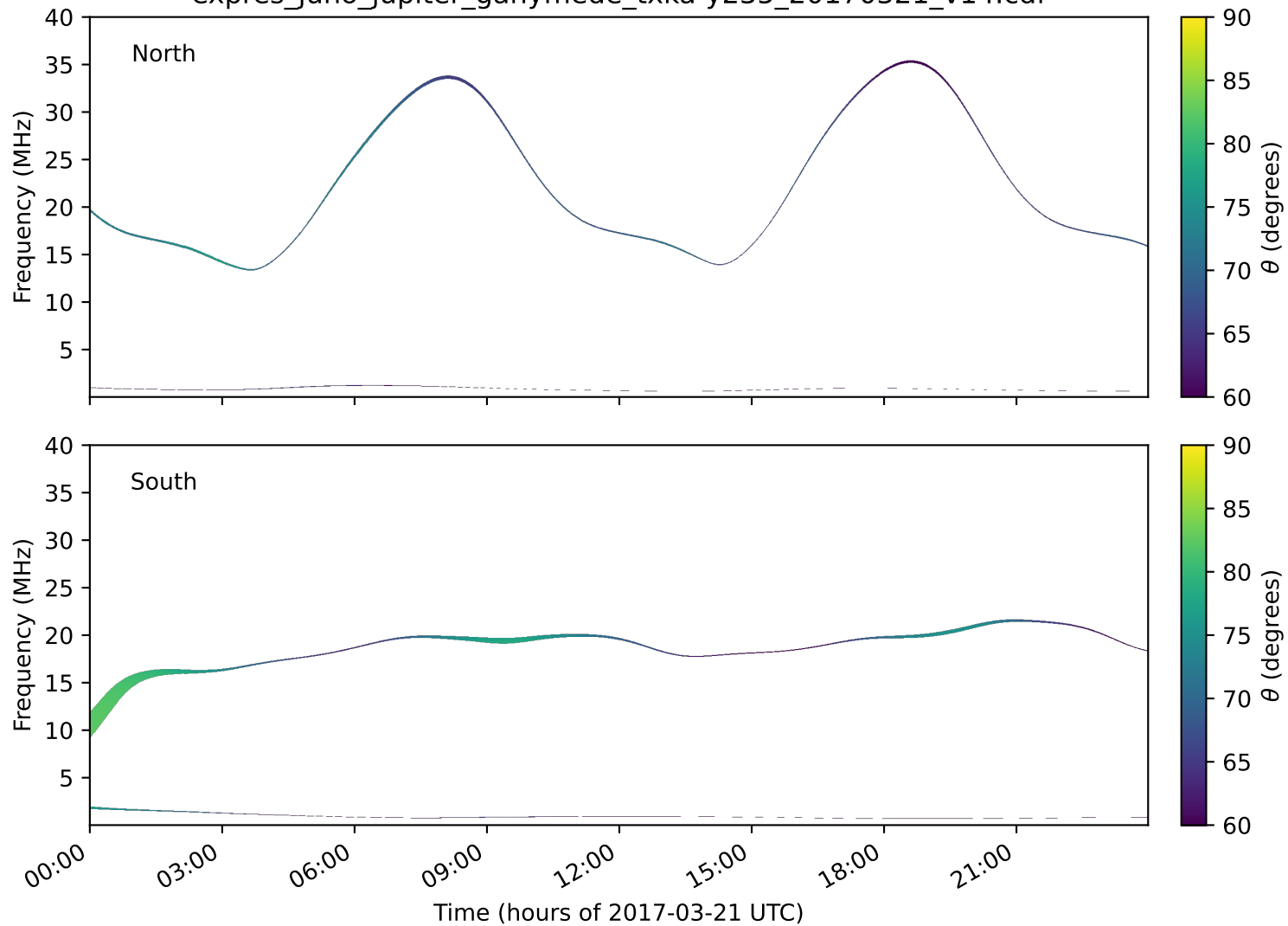
expres_juno_jupiter_ganymede_txka-y235_20170321_v14.cdf
