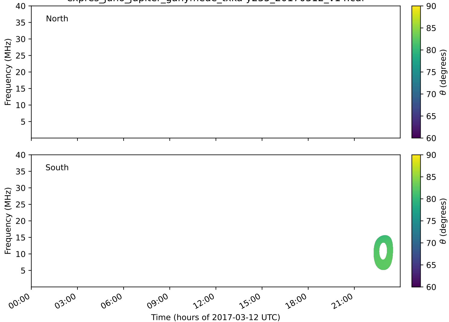
expres_juno_jupiter_ganymede_txka-y235_20170312_v14.cdf
