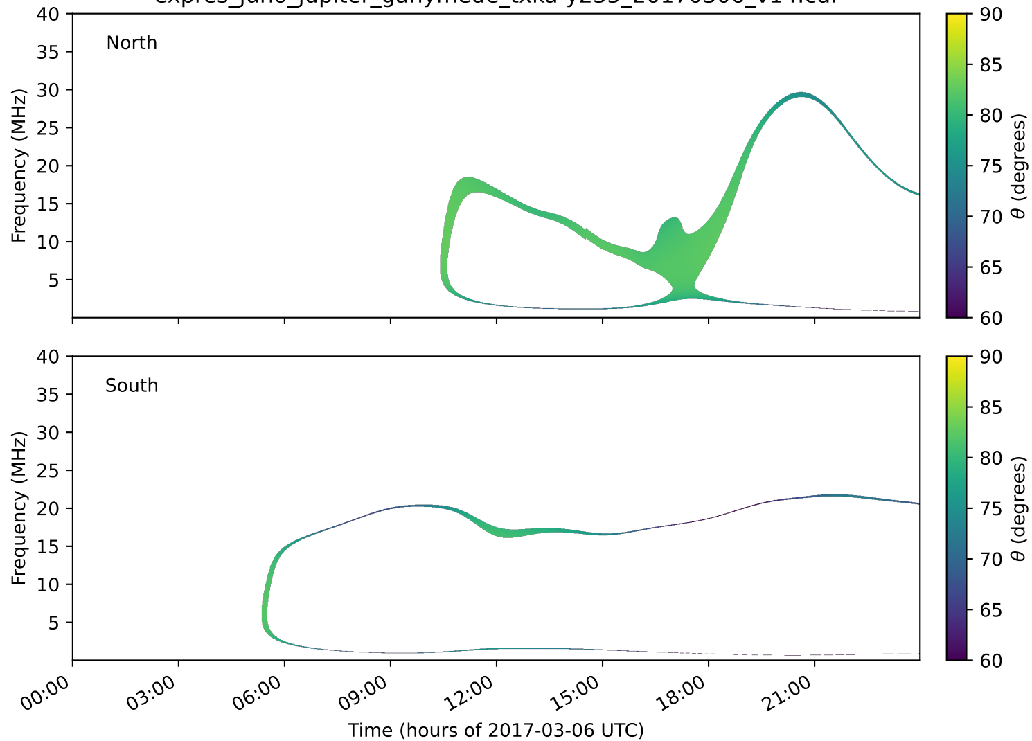
expres_juno_jupiter_ganymede_txka-y235_20170306_v14.cdf
