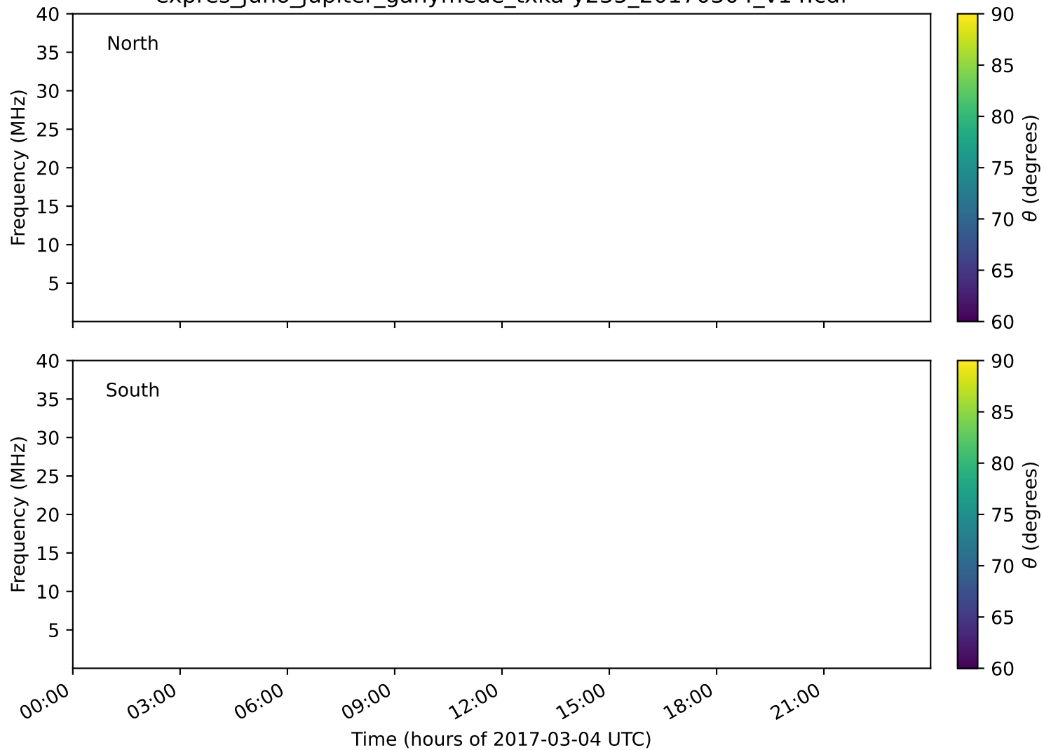
expres_juno_jupiter_ganymede_txka-y235_20170304_v14.cdf
