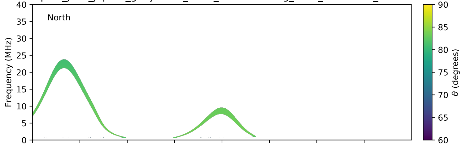
expres_juno_jupiter_ganymede_isaac_lossc-wid1deg_3kev_20170330_v01.cdf
