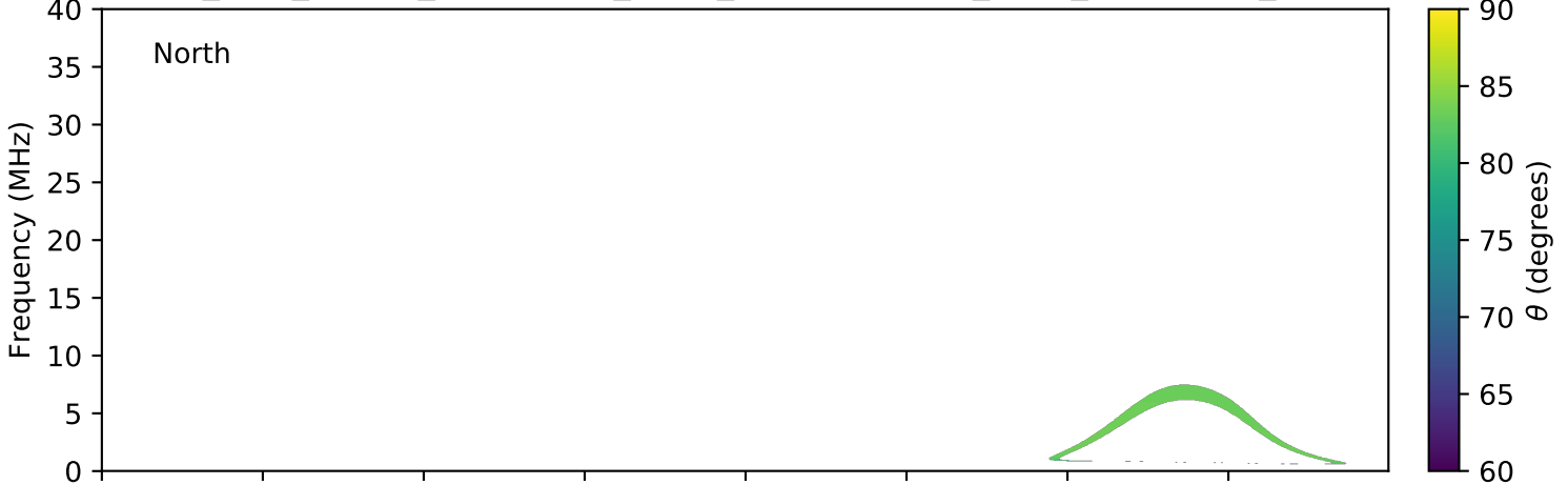
expres_juno_jupiter_ganymede_isaac_lossc-wid1deg_3kev_20170328_v01.cdf
