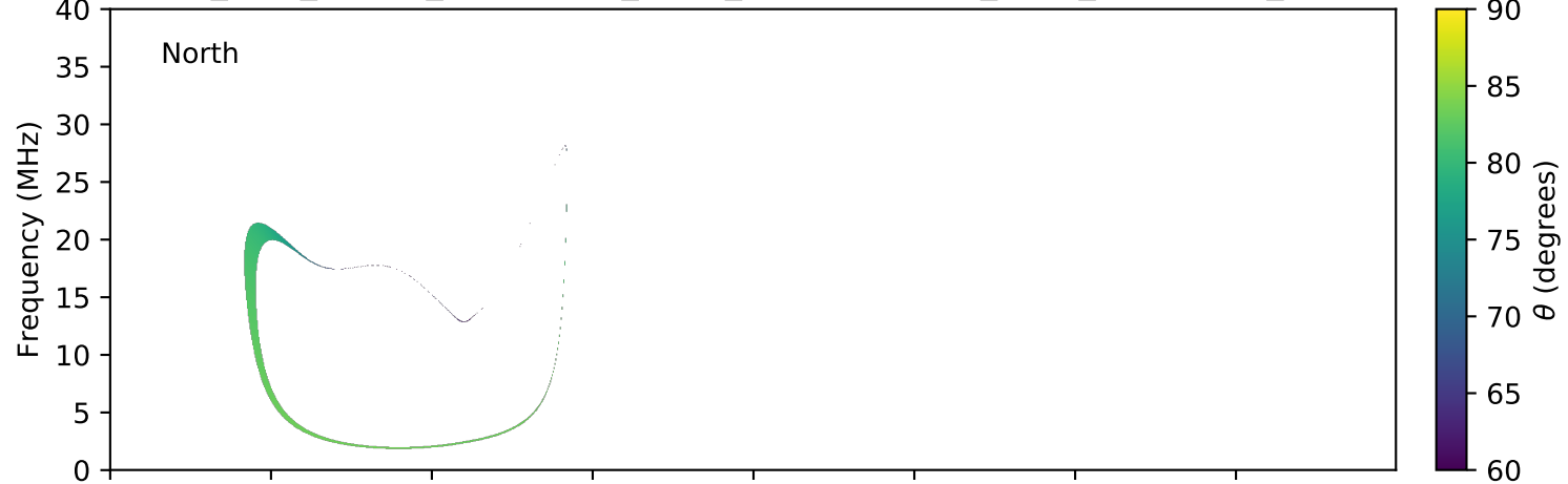
expres_juno_jupiter_ganymede_isaac_lossc-wid1deg_3kev_20170327_v01.cdf
