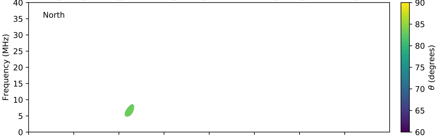
expres_juno_jupiter_ganymede_isaac_lossc-wid1deg_3kev_20170324_v01.cdf
