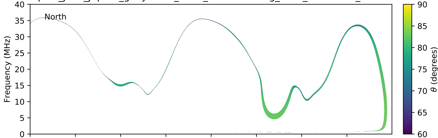
expres_juno_jupiter_ganymede_isaac_lossc-wid1deg_3kev_20170323_v01.cdf
