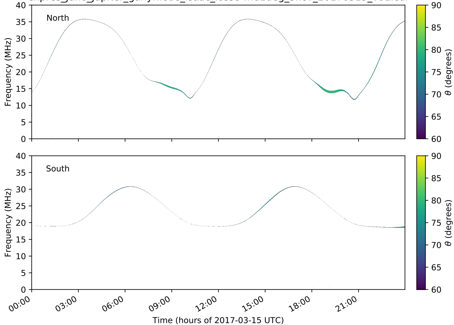
expres_juno_jupiter_ganymede_isaac_lossc-wid1deg_3kev_20170315_v01.cdf
