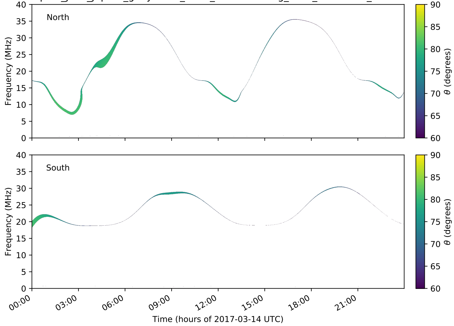
expres_juno_jupiter_ganymede_isaac_lossc-wid1deg_3kev_20170314_v01.cdf
