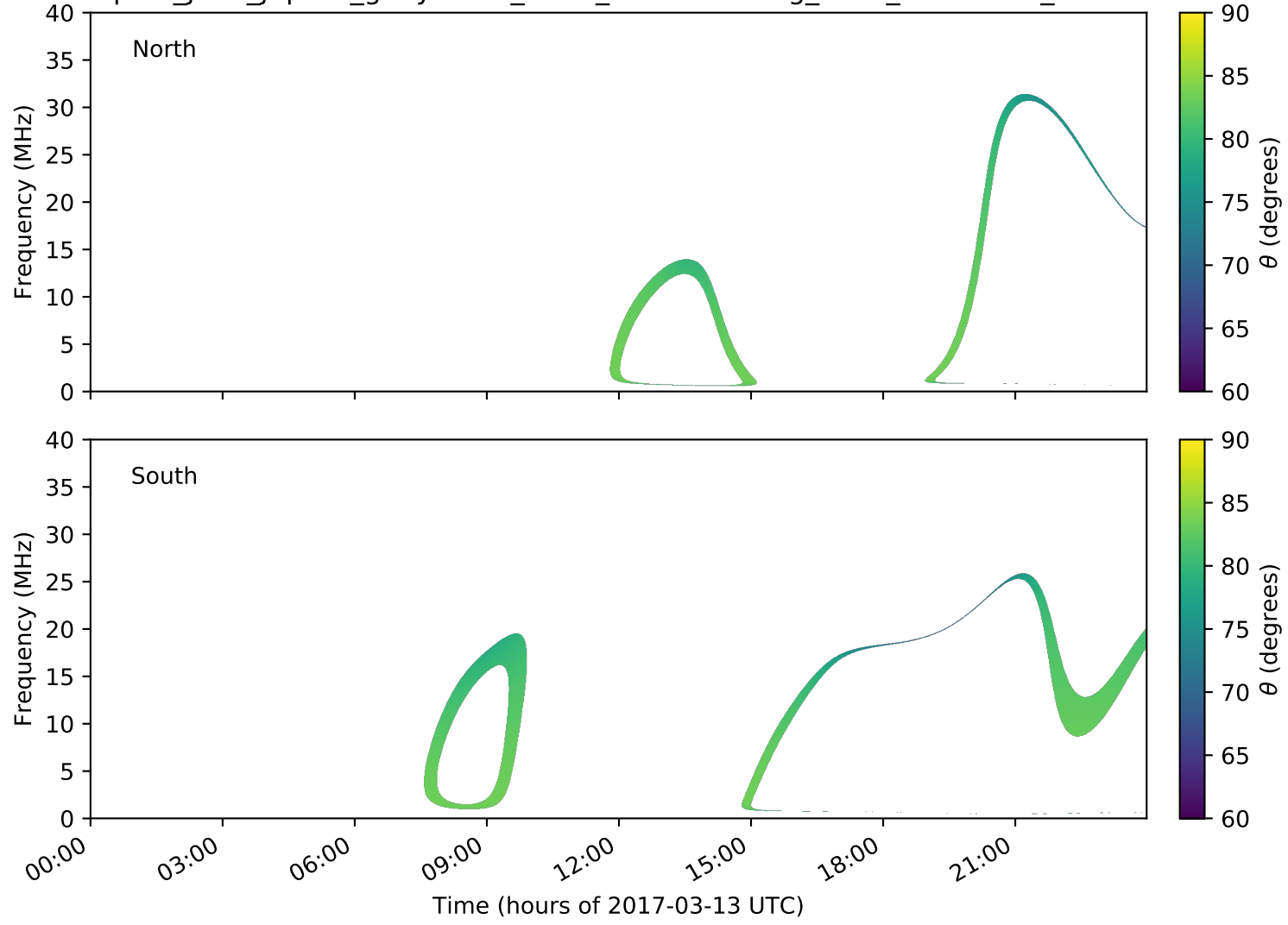
expres_juno_jupiter_ganymede_isaac_lossc-wid1deg_3kev_20170313_v01.cdf
