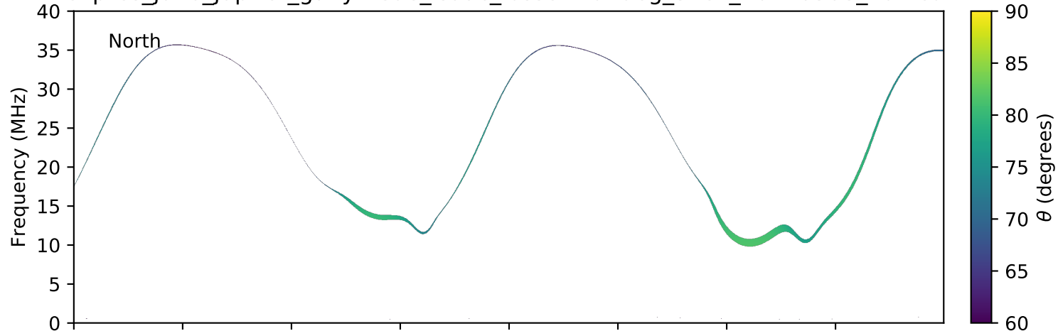
expres_juno_jupiter_ganymede_isaac_lossc-wid1deg_3kev_20170308_v01.cdf
