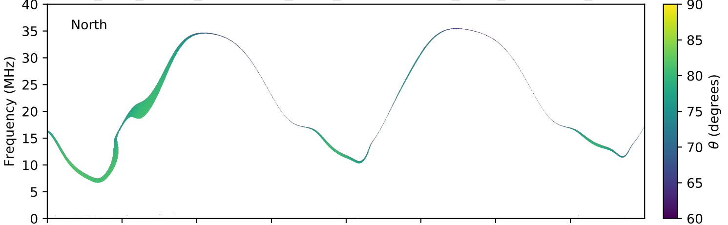
expres_juno_jupiter_ganymede_isaac_lossc-wid1deg_3kev_20170307_v01.cdf
