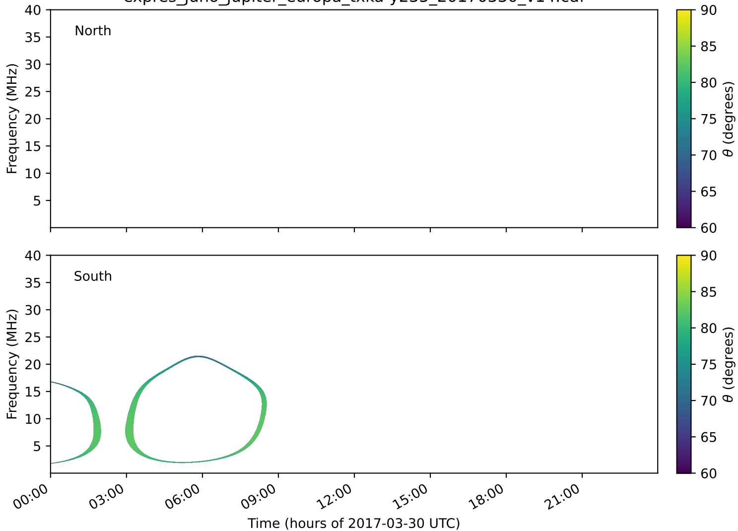
expres_juno_jupiter_europa_txka-y235_20170330_v14.cdf
