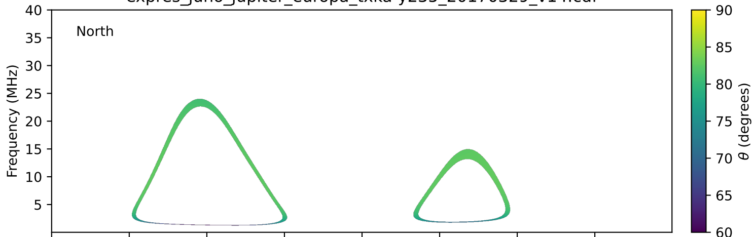
expres_juno_jupiter_europa_txka-y235_20170329_v14.cdf
