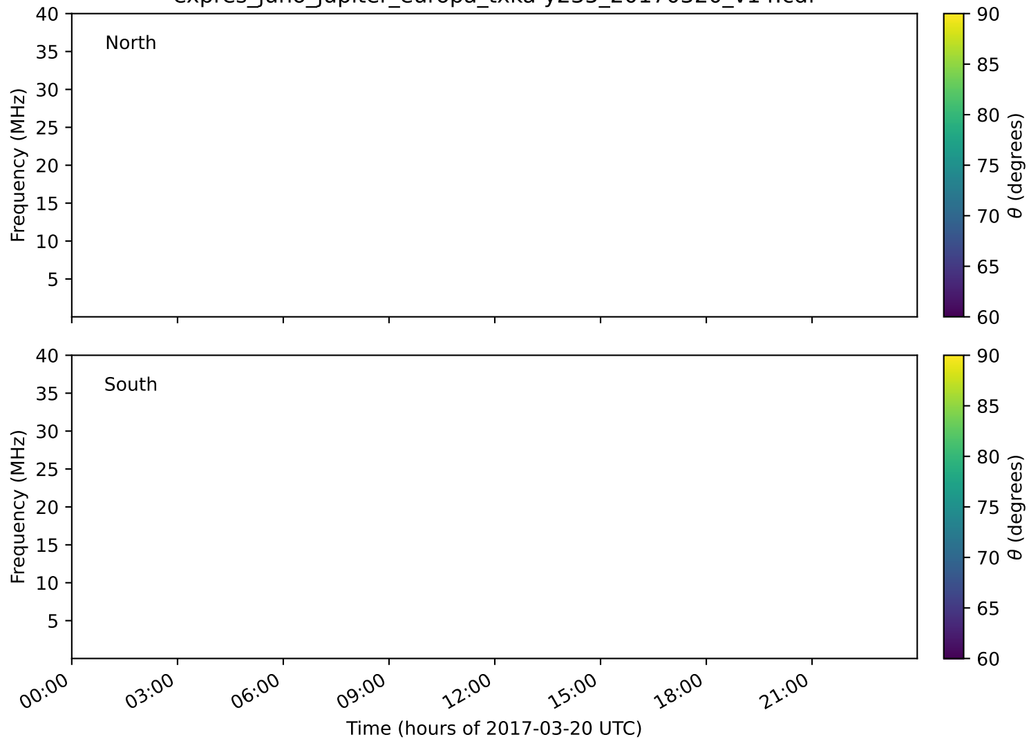
expres_juno_jupiter_europa_txka-y235_20170320_v14.cdf
