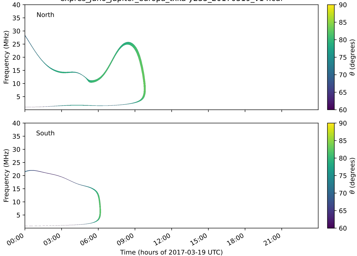
expres_juno_jupiter_europa_txka-y235_20170319_v14.cdf
