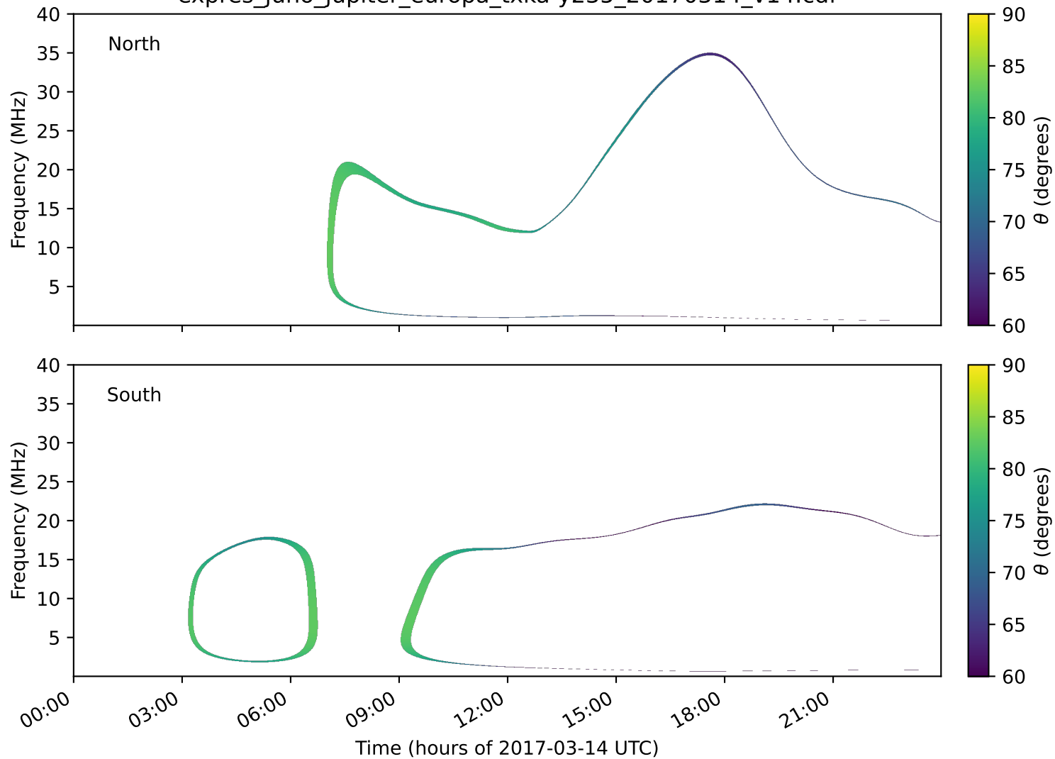
expres_juno_jupiter_europa_txka-y235_20170314_v14.cdf
